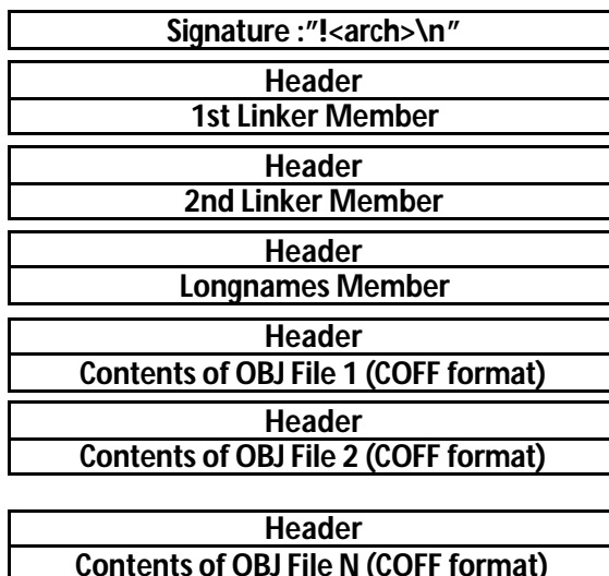
Figure 4. Archive File Structure
